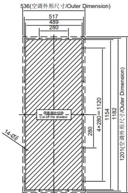
Figure 1-Cabinet Door Cutting Dimension
