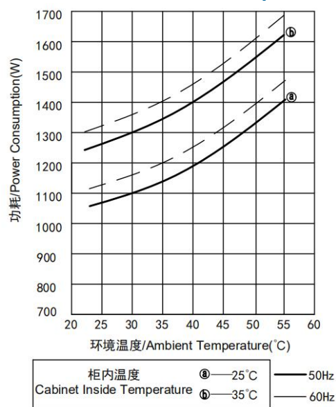
功耗曲线/Power Consumption Chart
