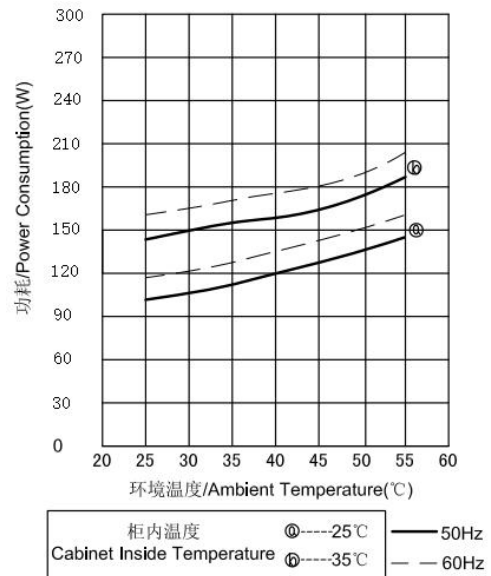
功耗曲线/Power Consumption Chart
