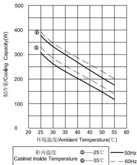
冷量曲线/Cooling Capacity Chart
