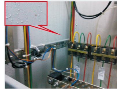
Before dehumidification the water drops on the cabinet is significantly
