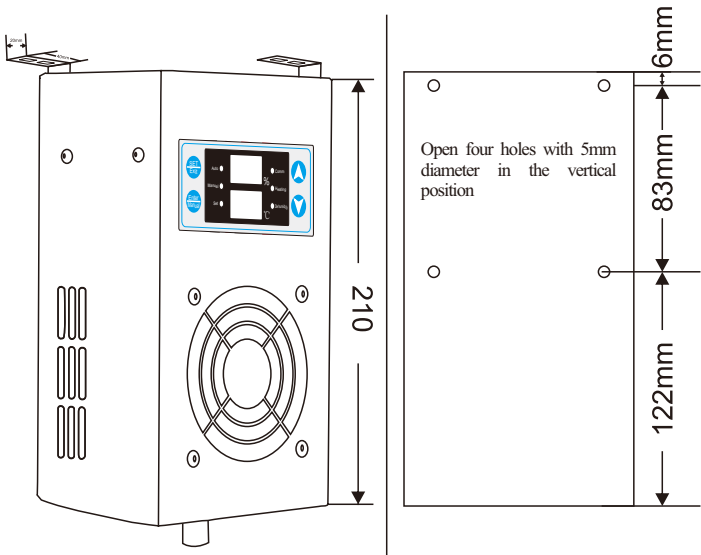
Dimensions : 210X115X67(mm) Wall-mounted installation hole diagram
